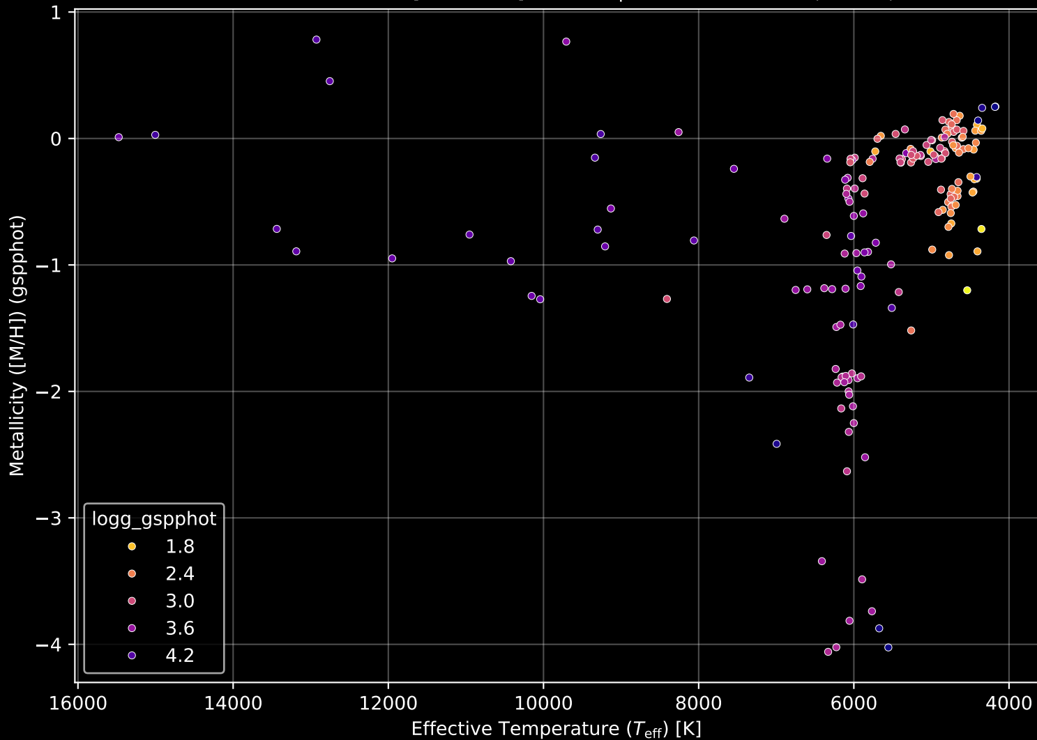
APOGEE DR17 Field: [N3201RRL] Stellar Population Parameters (n= 184)
