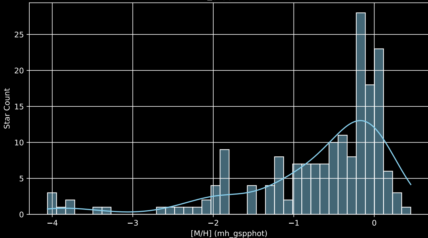
APOGEE DR17 Field: [N3201RRL [M/H] (mh_gspphot) (n= 182)
