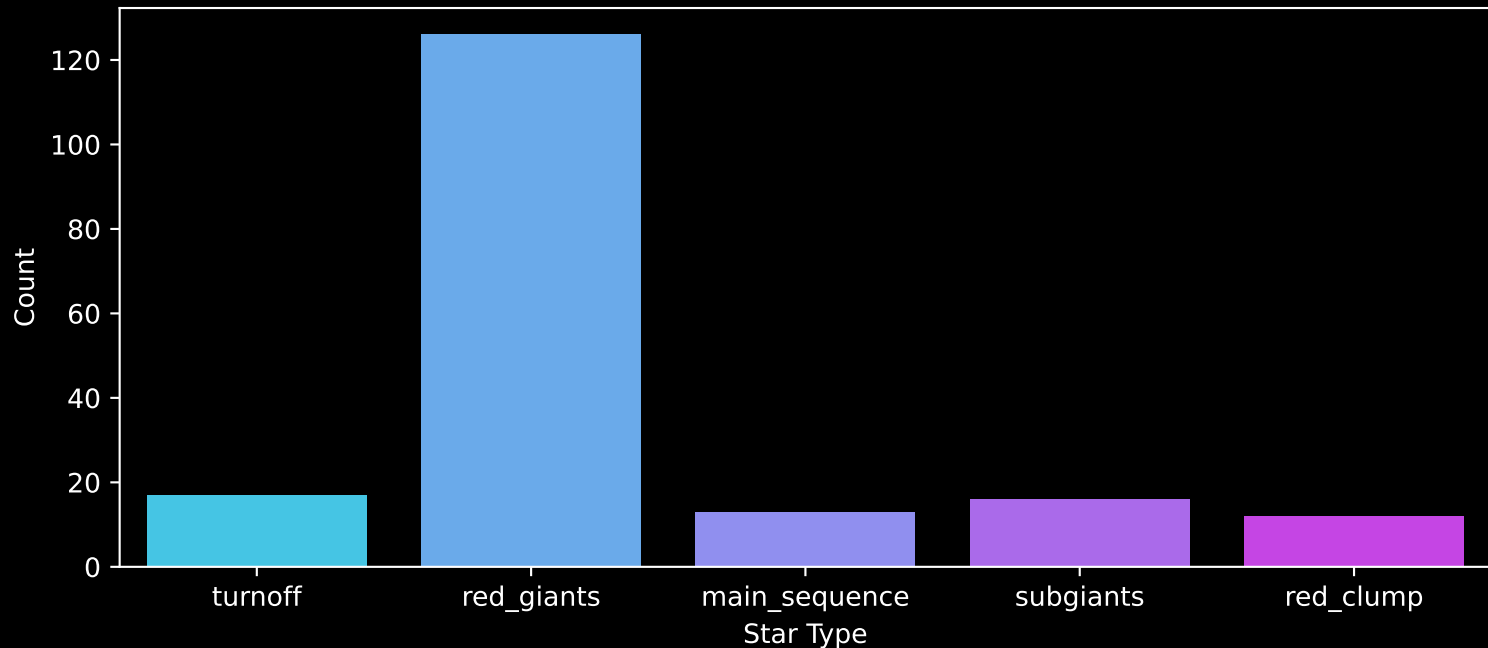
APOGEE DR17 Field: [N3201RRL] Count plot of Star Type
