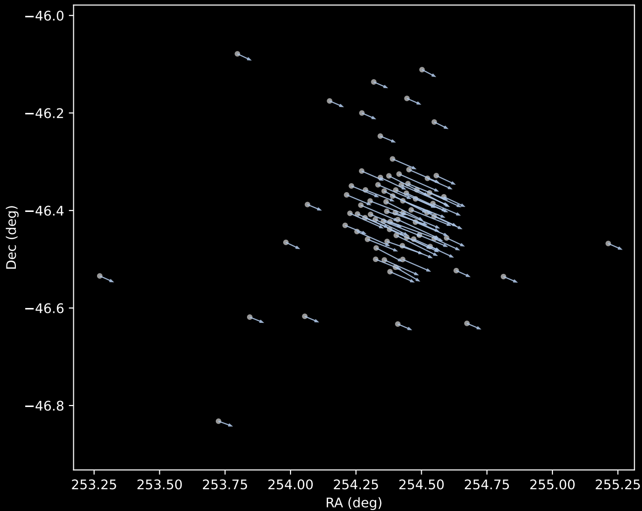
APOGEE DR17 Cluster 1 Proper Motion Vectors (n=80)
