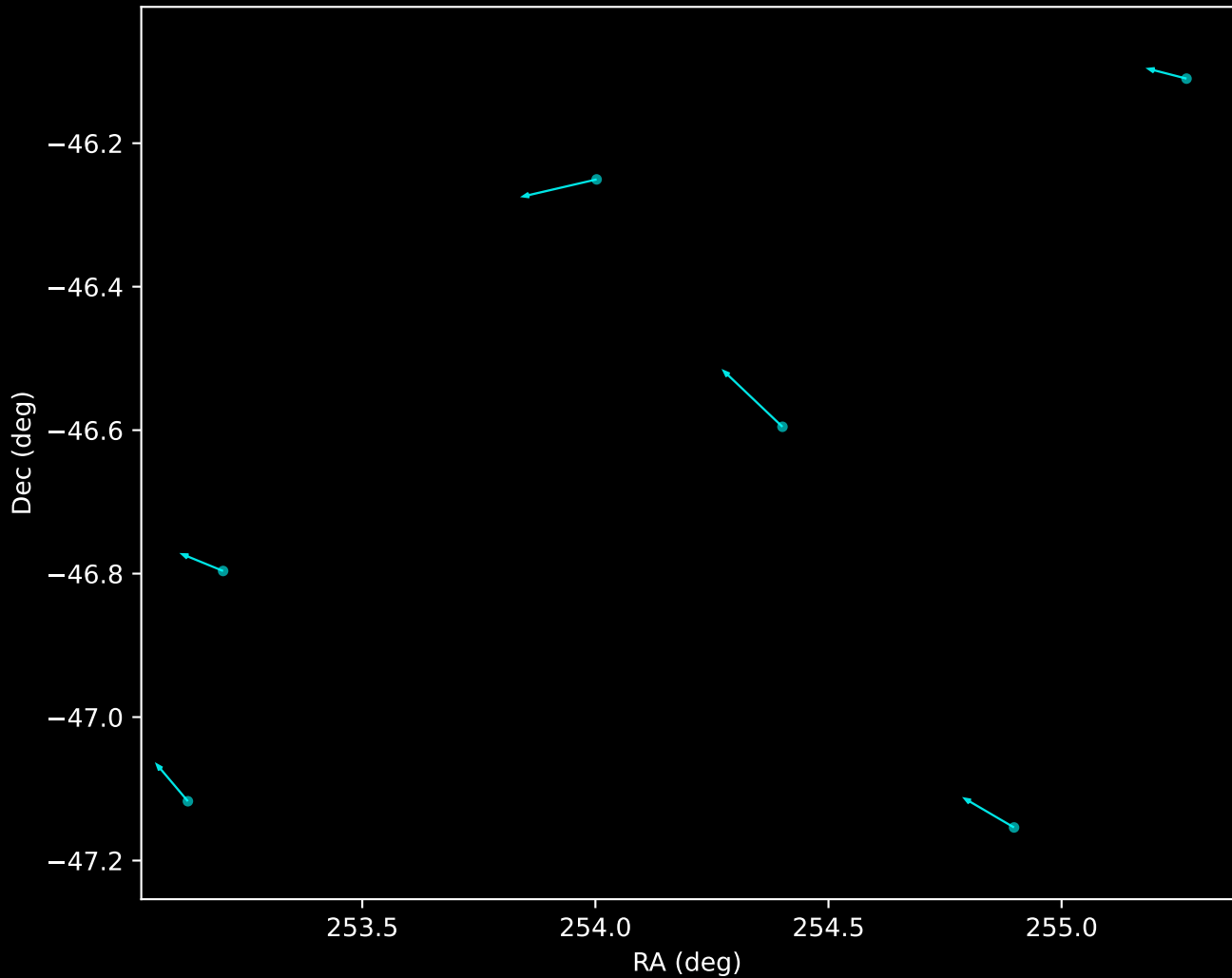
APOGEE DR17 Noise Stream Proper Motion Vectors (n=6)
