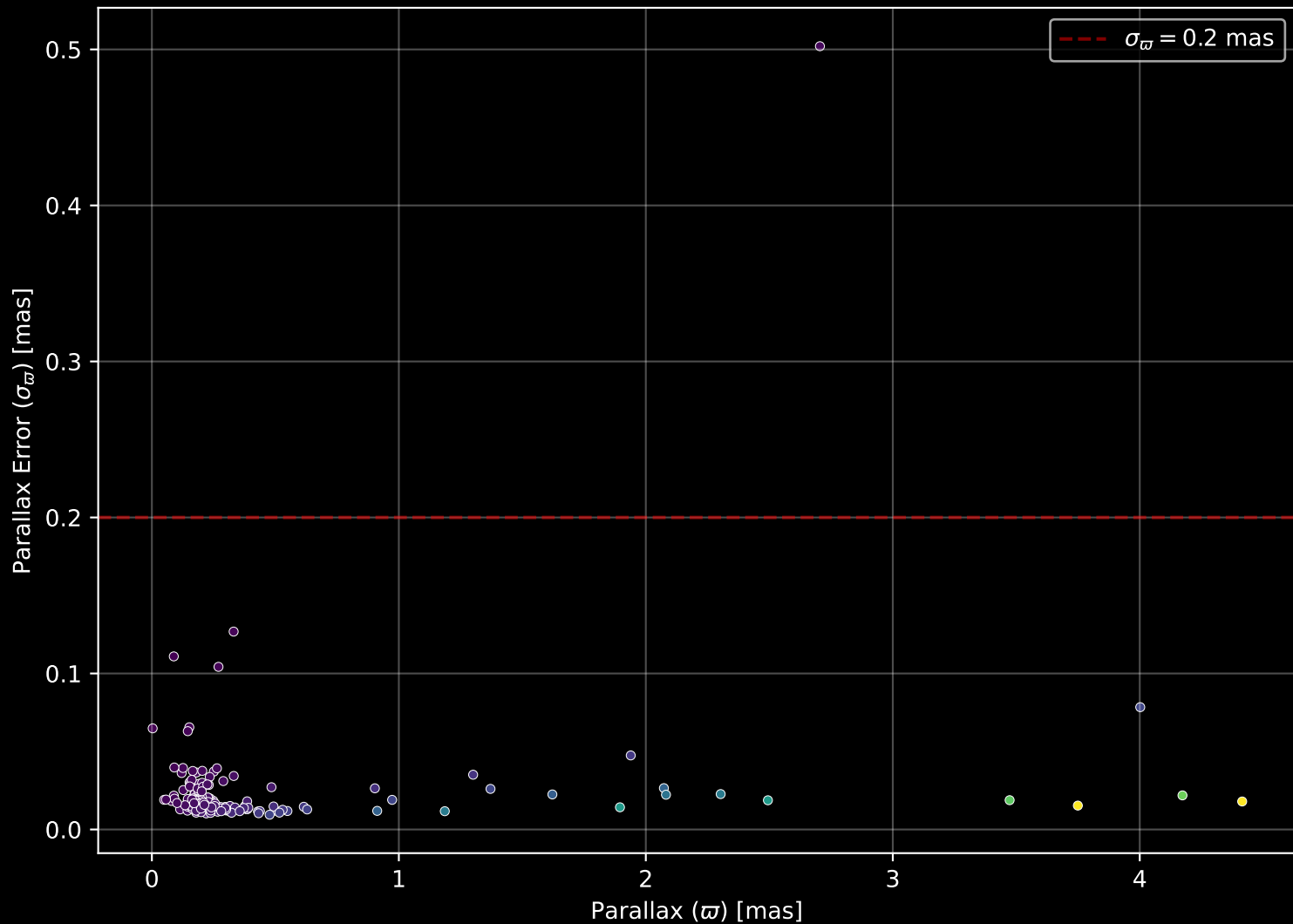
APOGEE DR17 Field: [N3201RRL] Parallax Quality (n= 184)
