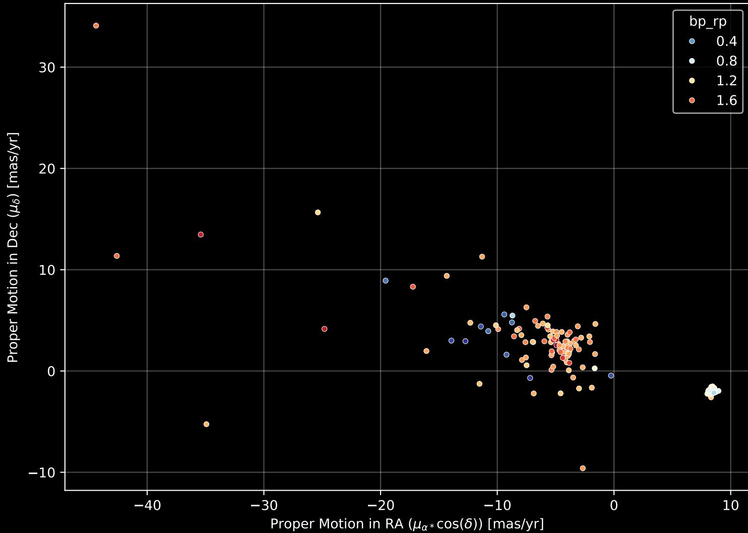
APOGEE DR17 Field: [N3201RRL] Proper Motion Diagram (n= 184)
