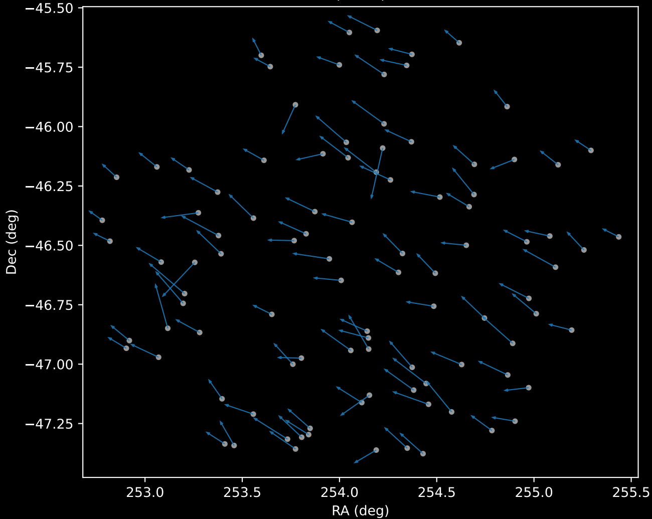
APOGEE DR17 Cluster 0 Proper Motion Vectors (n=98)
