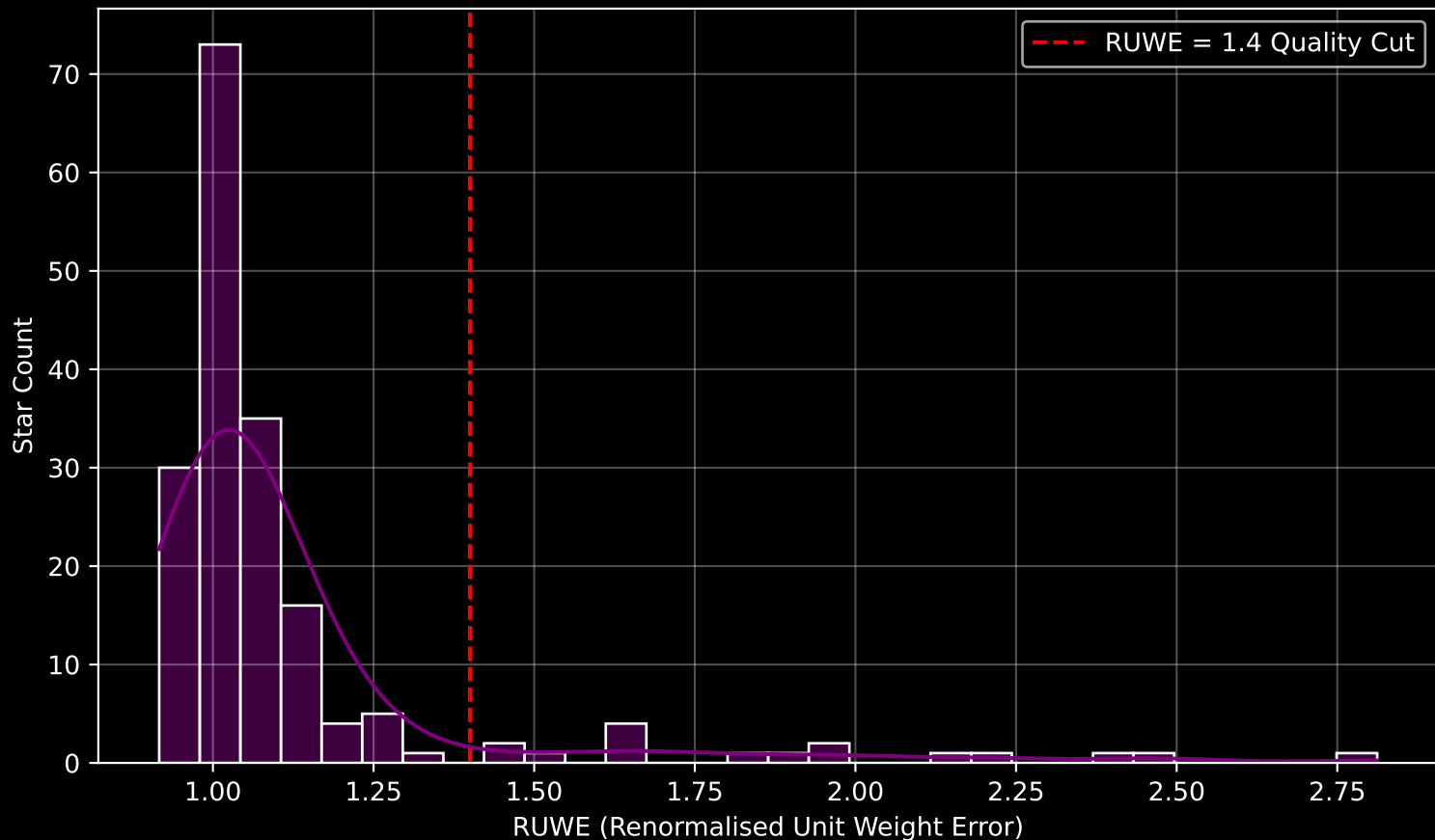
GAPOGEE DR17 Field [N3201RRL] RUWE Distribution (n= 180)
